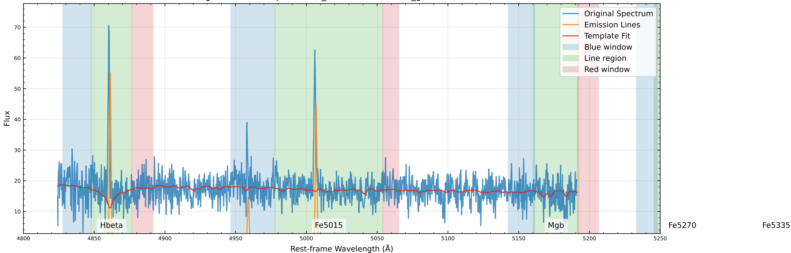
Original Data Comparison (v_star=-35.6 km/s, v_gas=-57.0 km/s)
