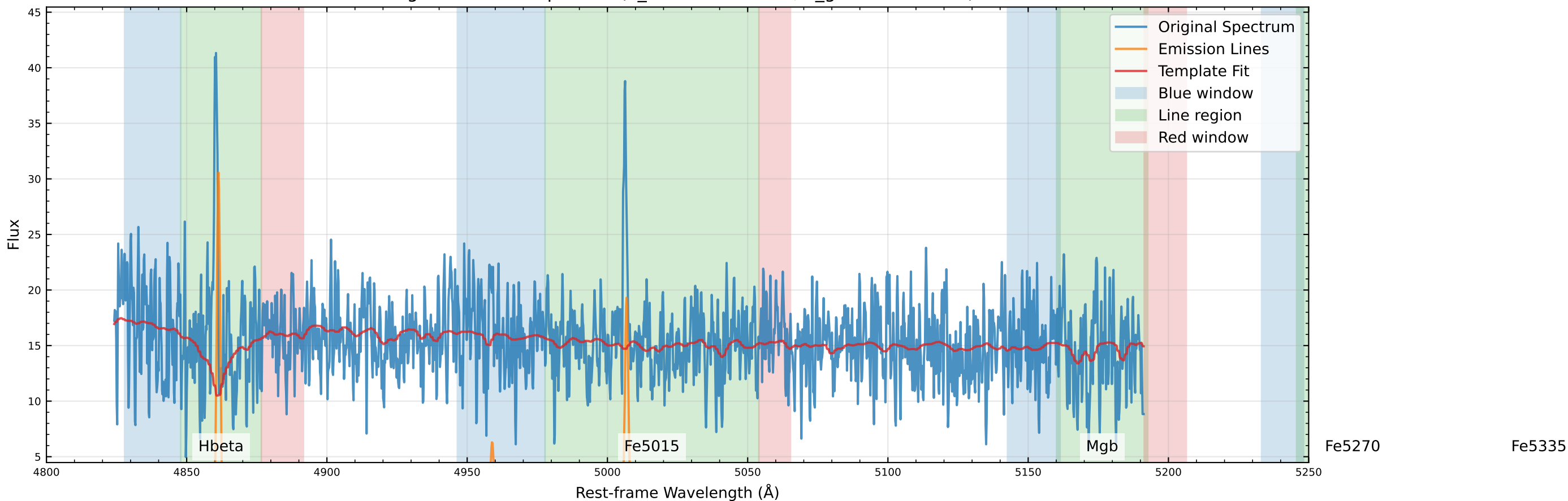
Original Data Comparison (v_star=-59.8 km/s, v_gas=-50.3 km/s)
