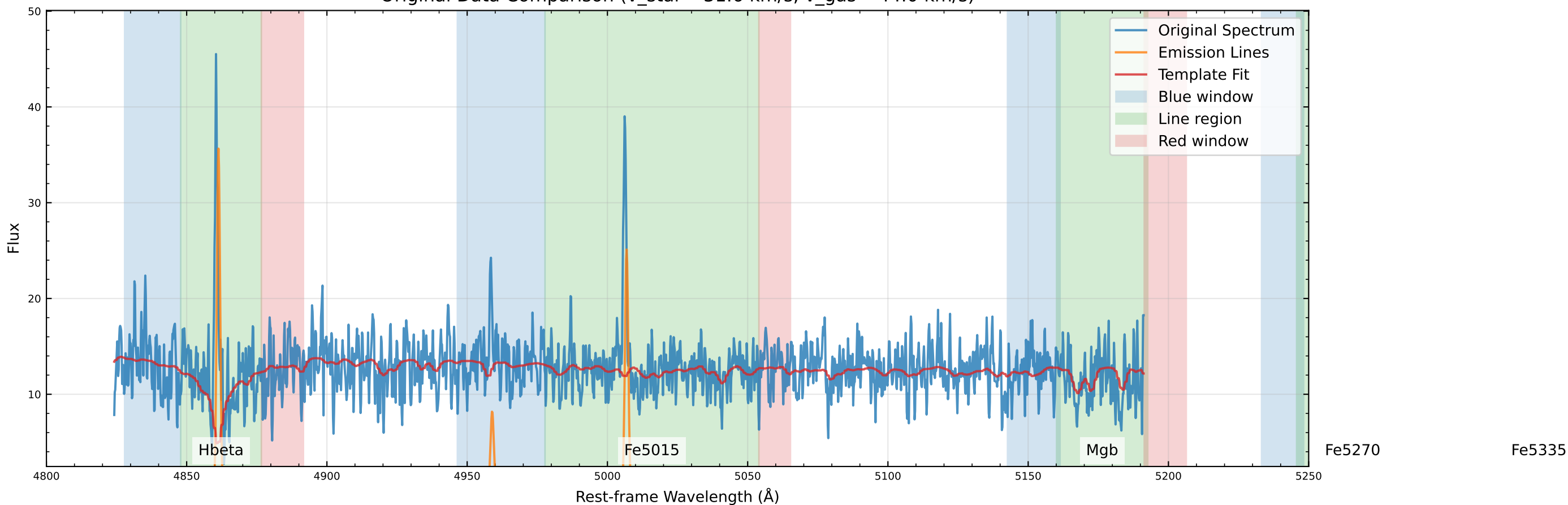
Original Data Comparison (v_star=-31.6 km/s, v_gas=-44.0 km/s)
