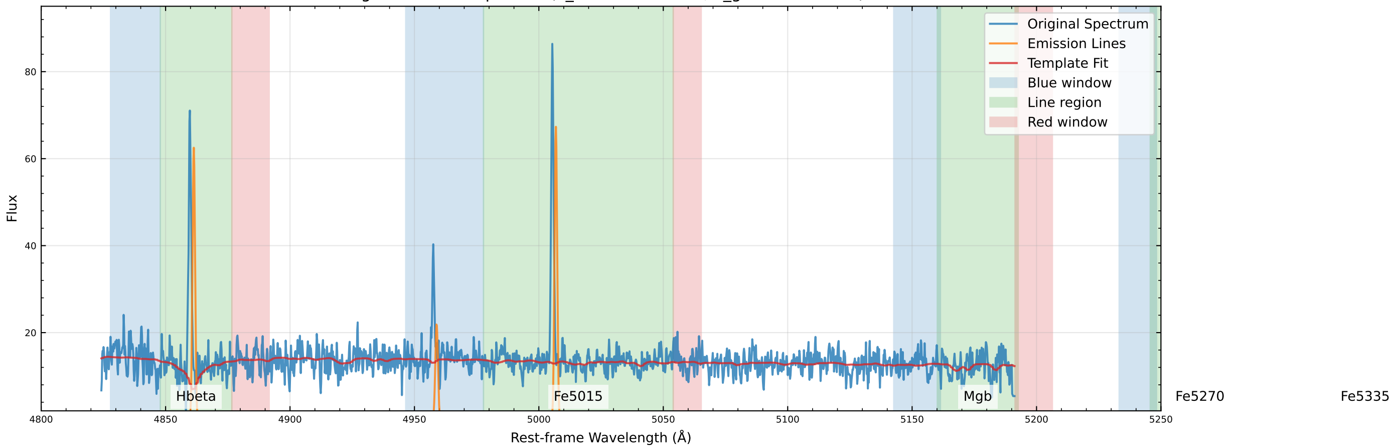
Original Data Comparison (v_star=-98.3 km/s, v_gas=-88.4 km/s)
