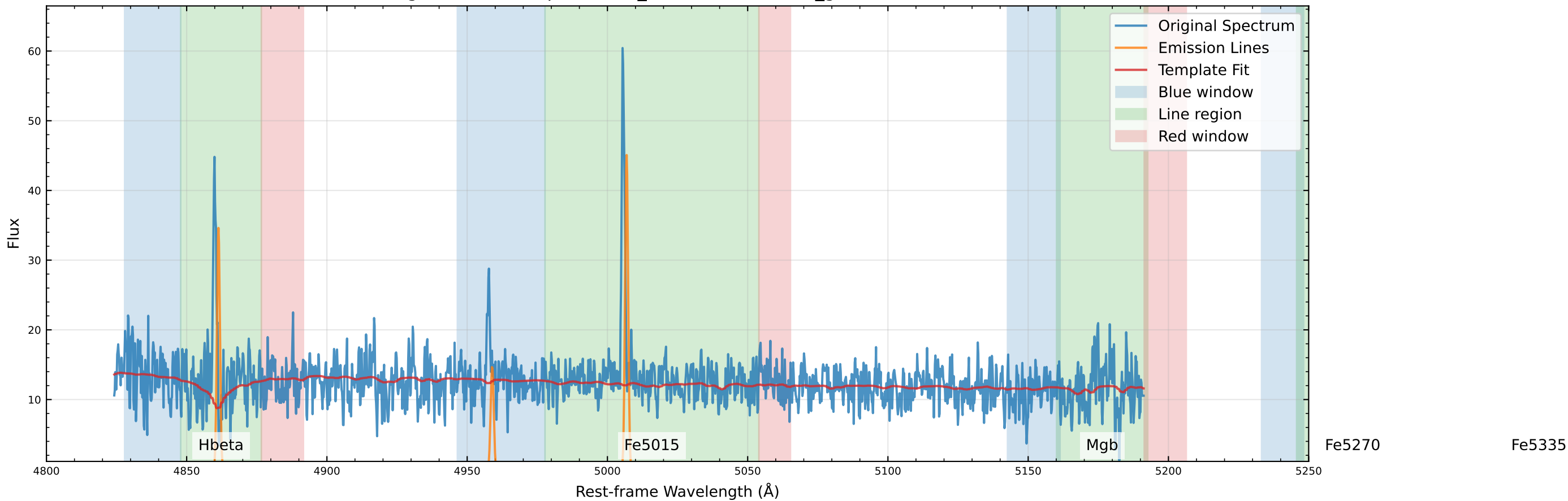
Original Data Comparison (v_star=-71.9 km/s, v_gas=-76.9 km/s)
