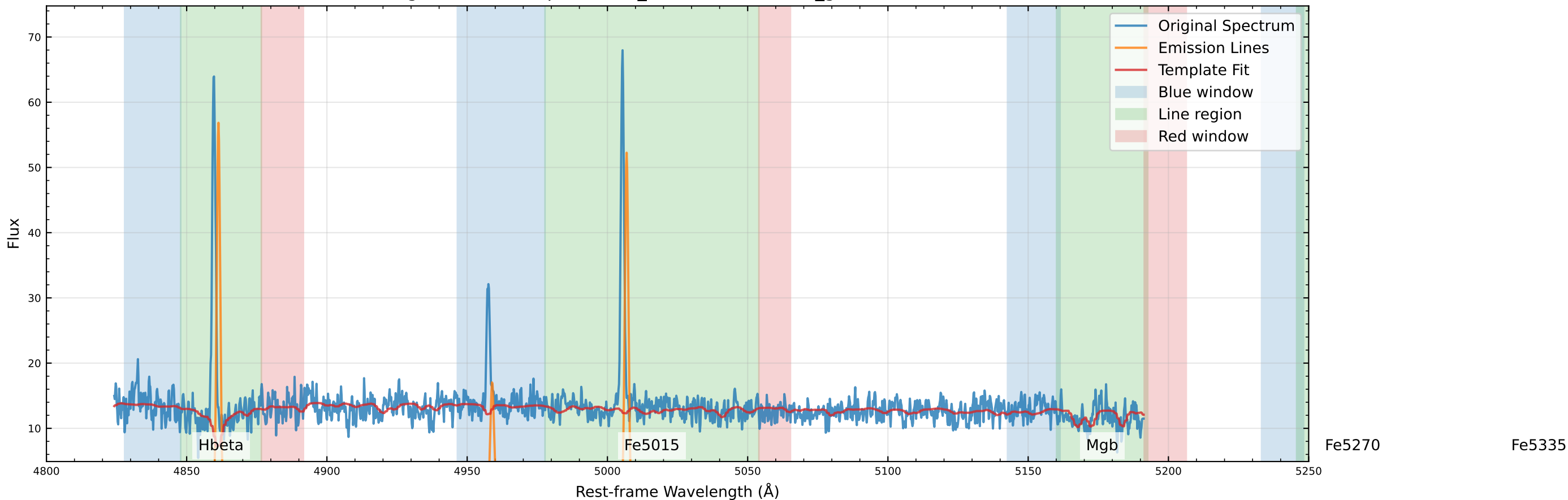
Original Data Comparison (v_star=-90.6 km/s, v_gas=-94.7 km/s)
