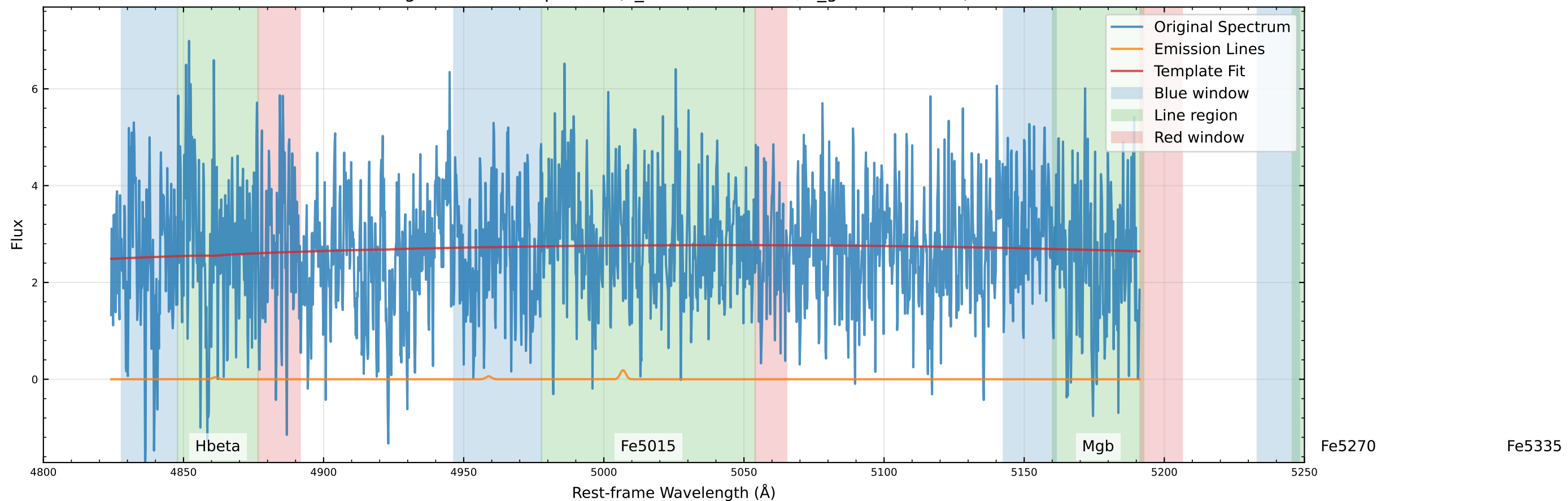
Original Data Comparison (v_star=113.9 km/s, v_gas=99.3 km/s)
