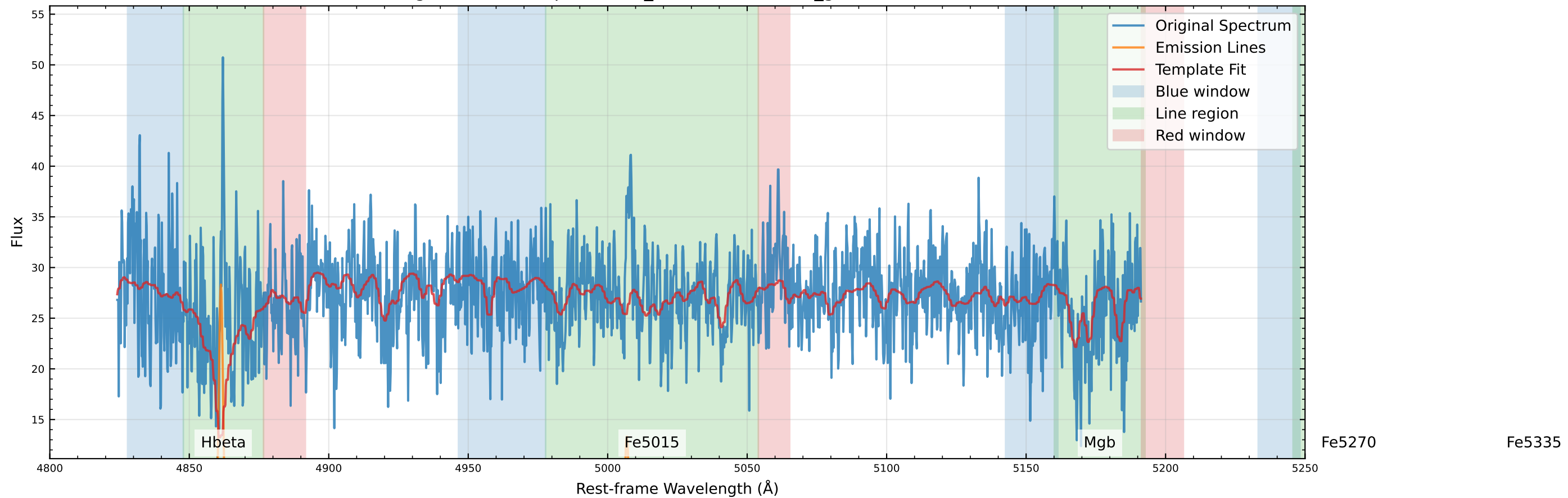
Original Data Comparison (v_star=44.7 km/s, v_gas=46.3 km/s)
