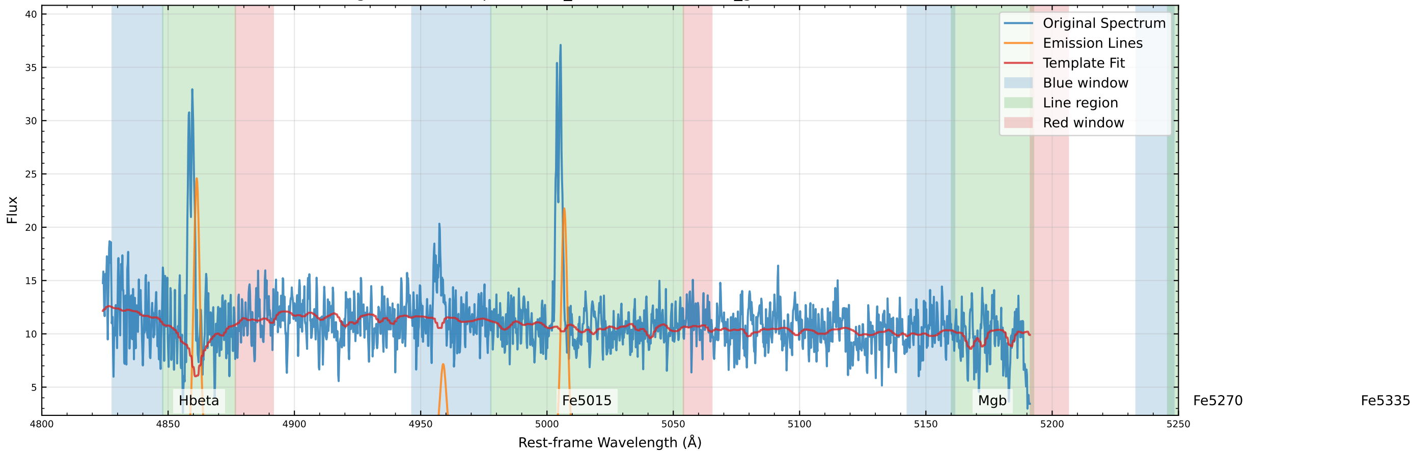
Original Data Comparison (v_star=-126.8 km/s, v_gas=-127.9 km/s)
