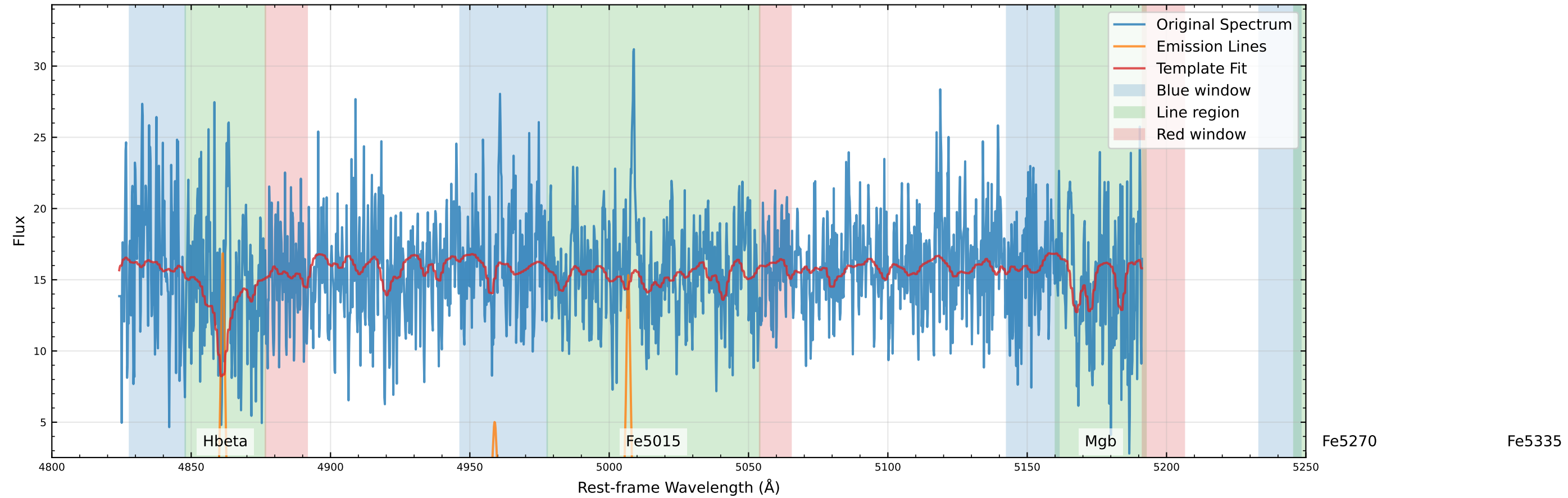
Original Data Comparison (v_star=76.0 km/s, v_gas=106.3 km/s)
