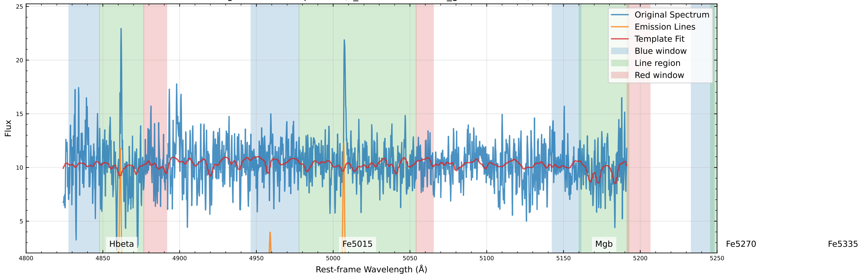
Original Data Comparison (v_star=27.5 km/s, v_gas=36.3 km/s)
