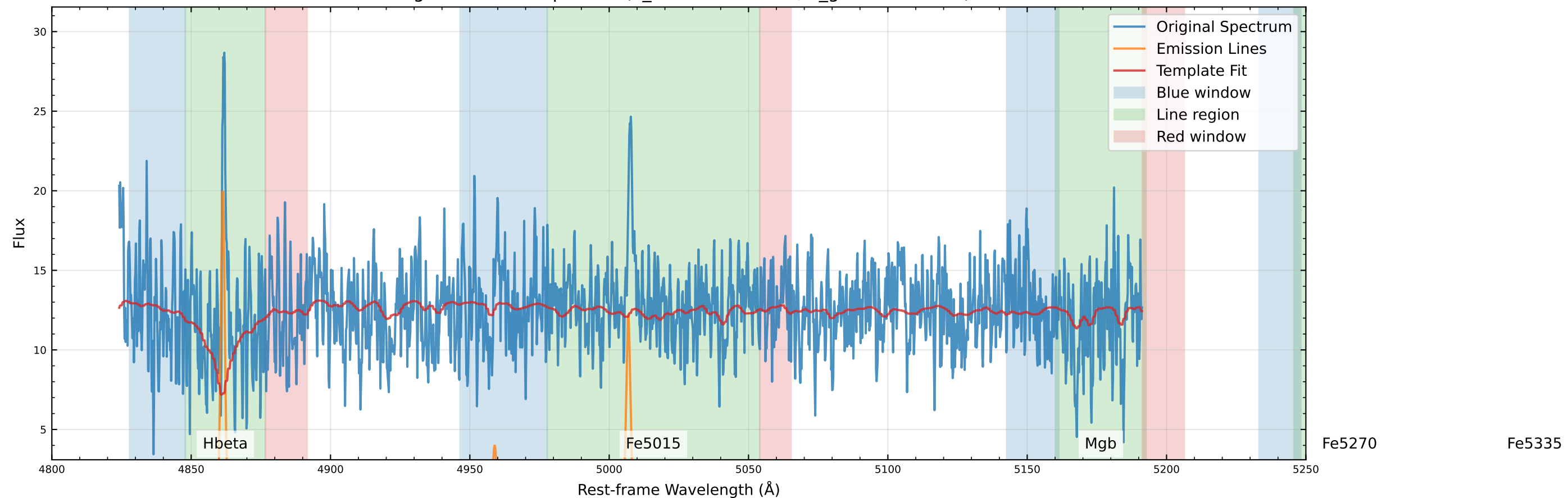
Original Data Comparison (v_star=-11.9 km/s, v_gas=35.7 km/s)
