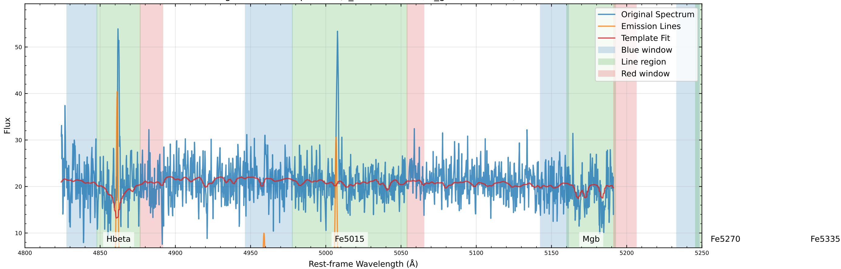
Original Data Comparison (v_star=4.5 km/s, v_gas=52.5 km/s)
