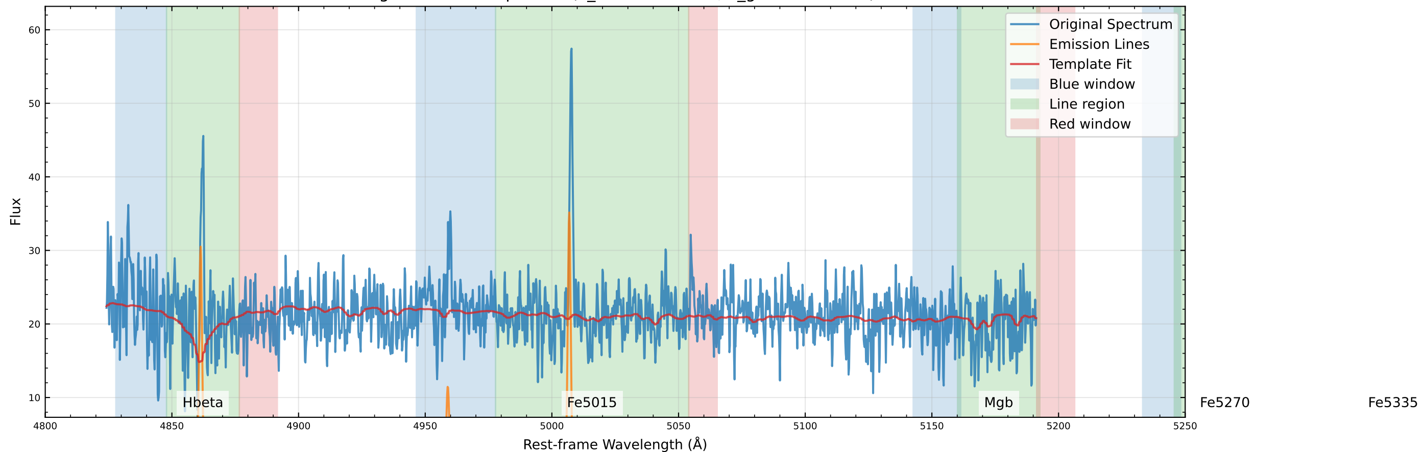
Original Data Comparison (v_star=-4.1 km/s, v_gas=44.4 km/s)
