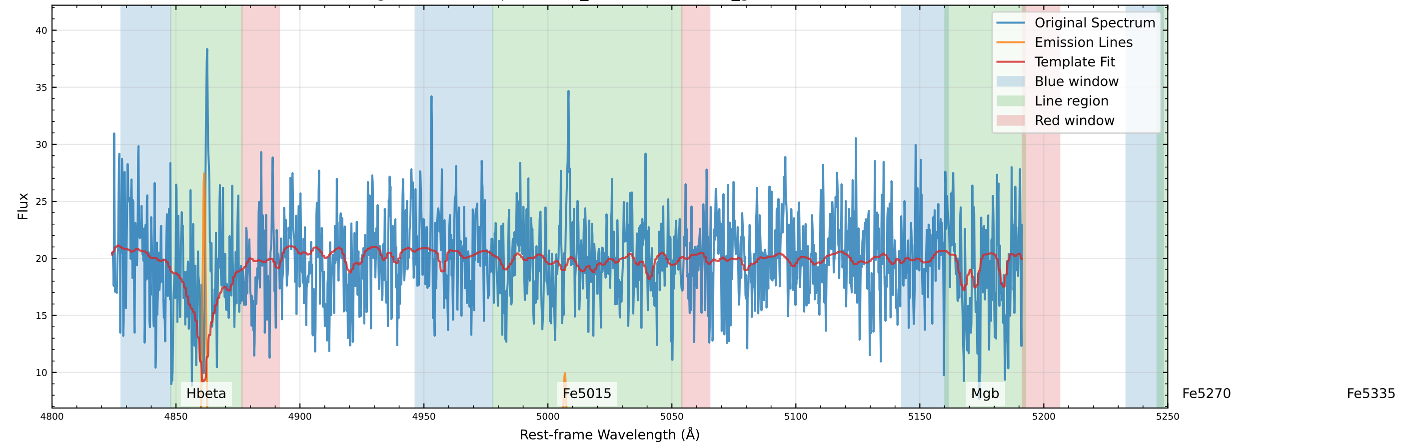
Original Data Comparison (v_star=62.4 km/s, v_gas=80.6 km/s)
