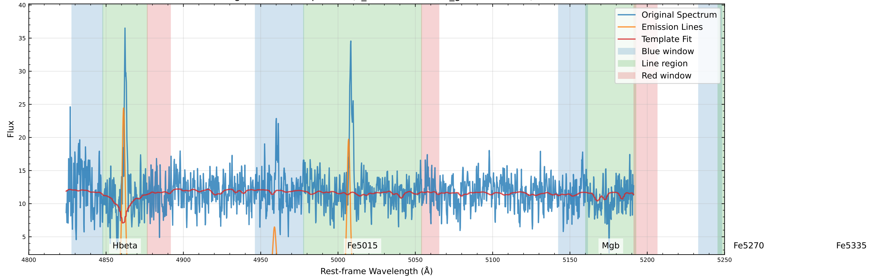
Original Data Comparison (v_star=0.8 km/s, v_gas=82.4 km/s)
