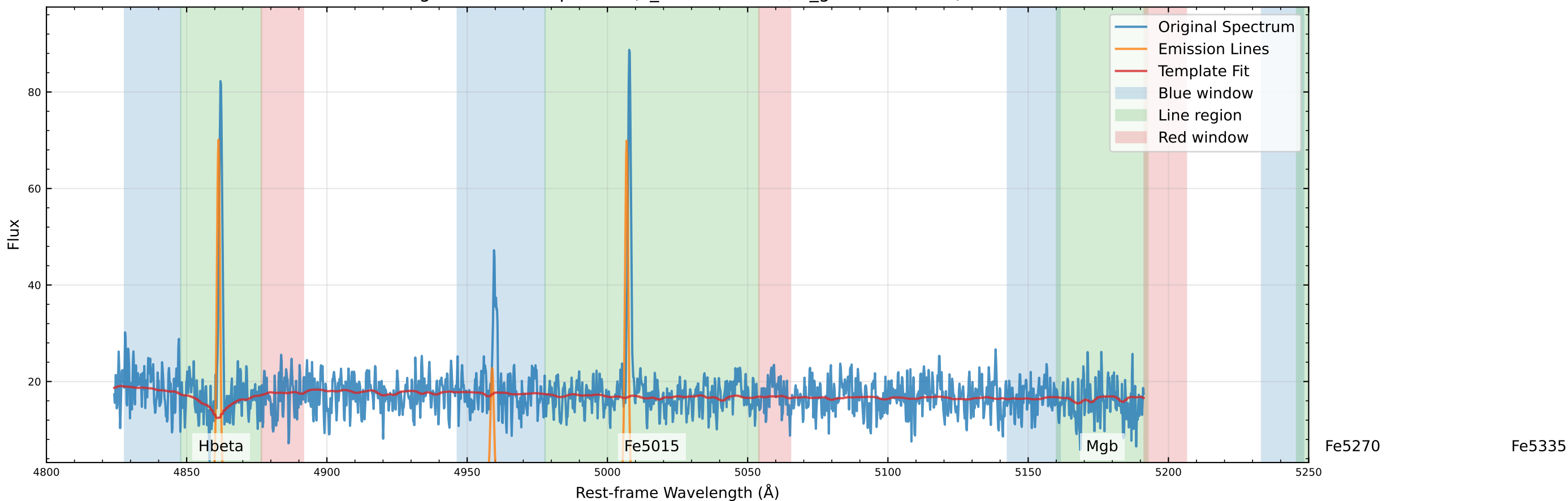
Original Data Comparison (v_star=8.4 km/s, v_gas=53.4 km/s)
