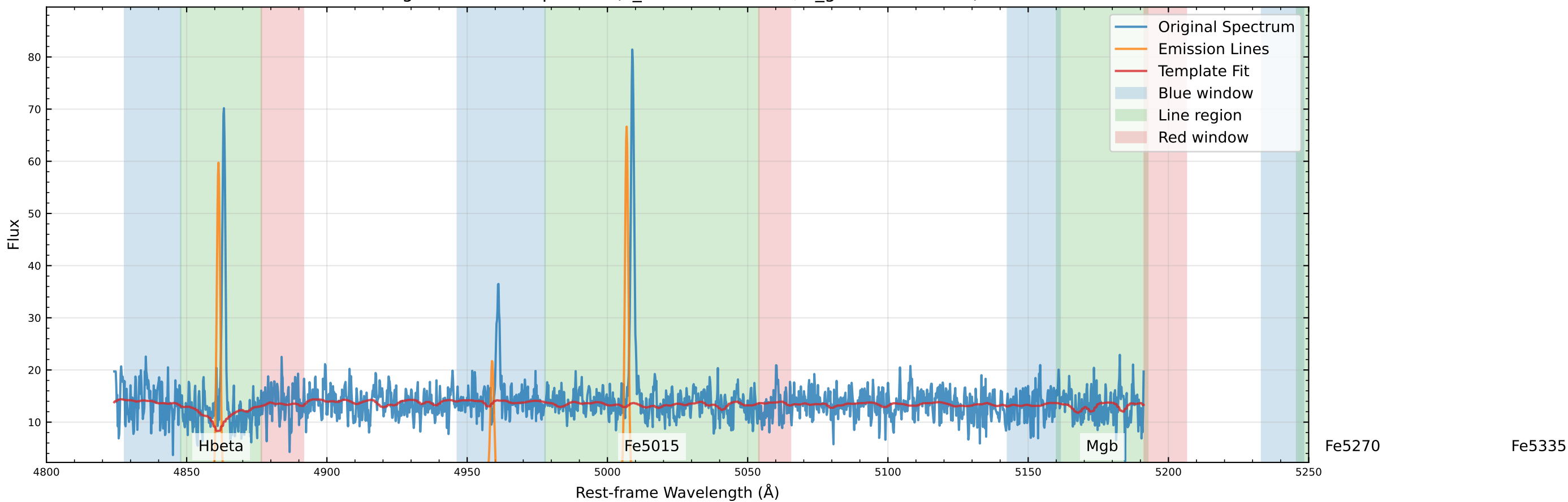
Original Data Comparison (v_star=109.2 km/s, v_gas=121.5 km/s)
