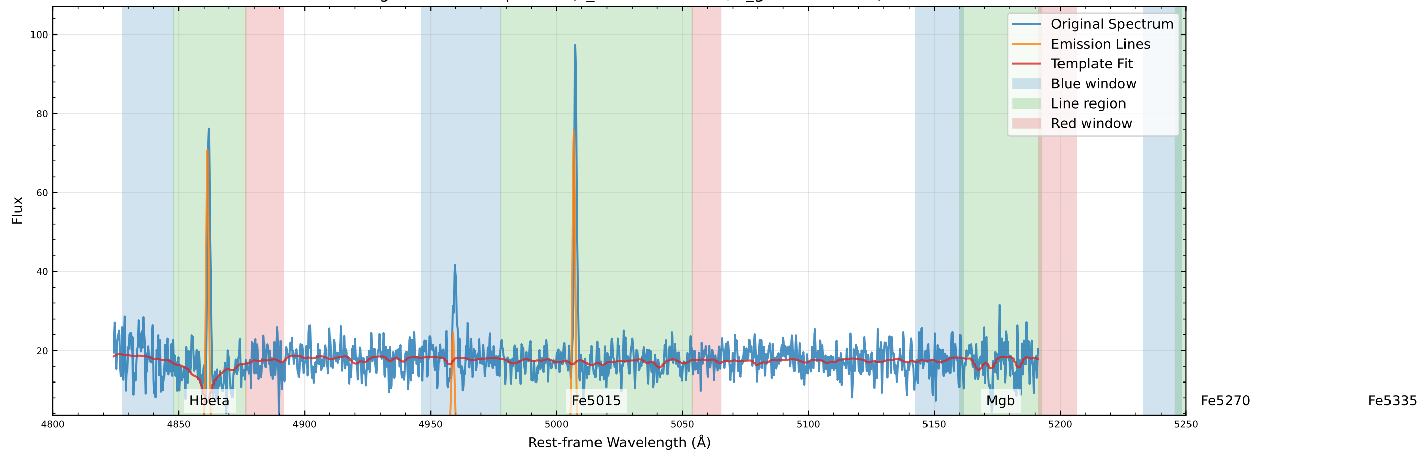
Original Data Comparison (v_star=-16.5 km/s, v_gas=38.0 km/s)
