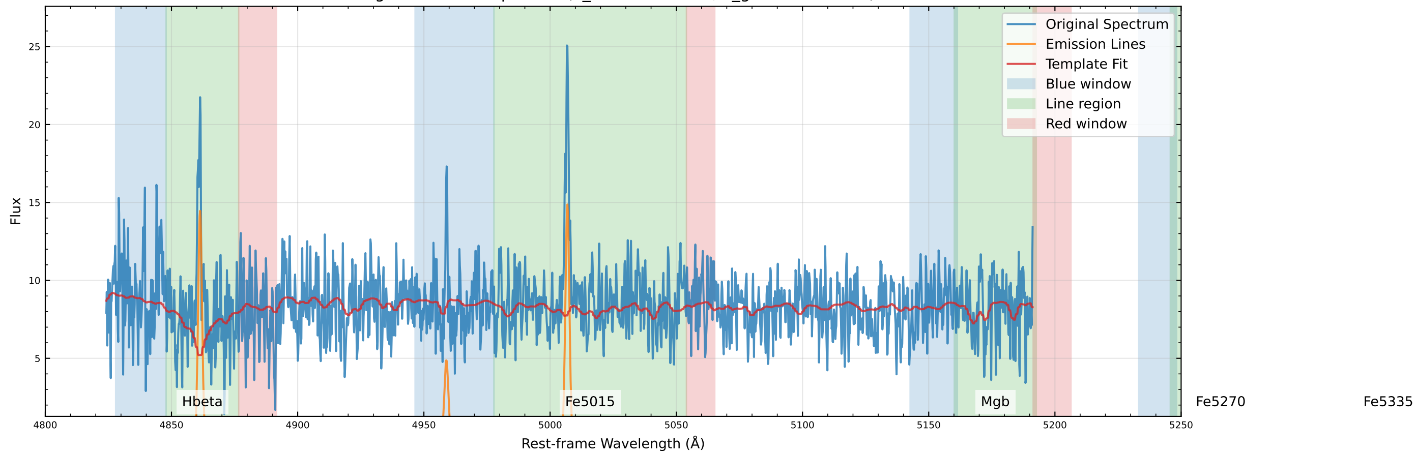
Original Data Comparison (v_star=-0.5 km/s, v_gas=-10.6 km/s)
