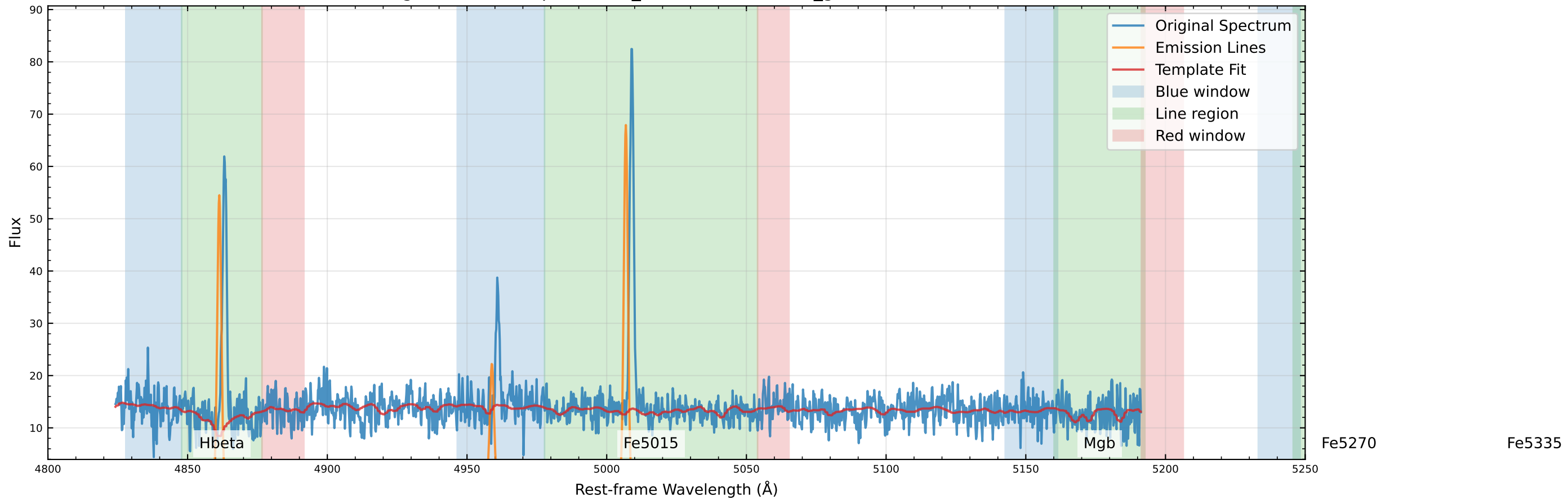
Original Data Comparison (v_star=108.7 km/s, v_gas=122.5 km/s)
