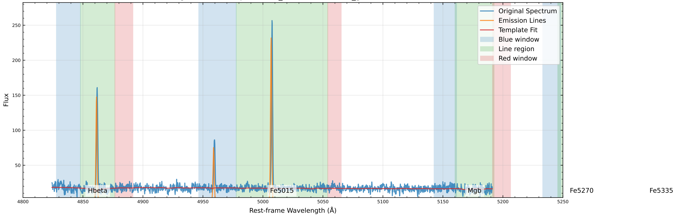
Original Data Comparison (v_star=29.3 km/s, v_gas=41.8 km/s)
