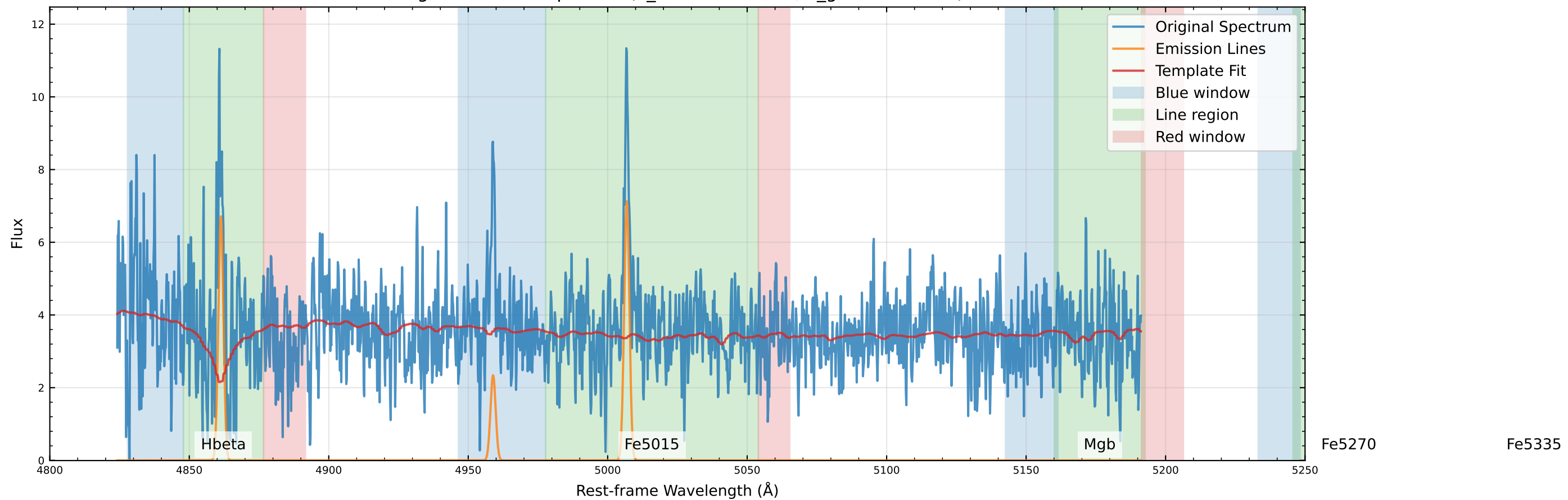
Original Data Comparison (v_star=41.5 km/s, v_gas=-7.1 km/s)
