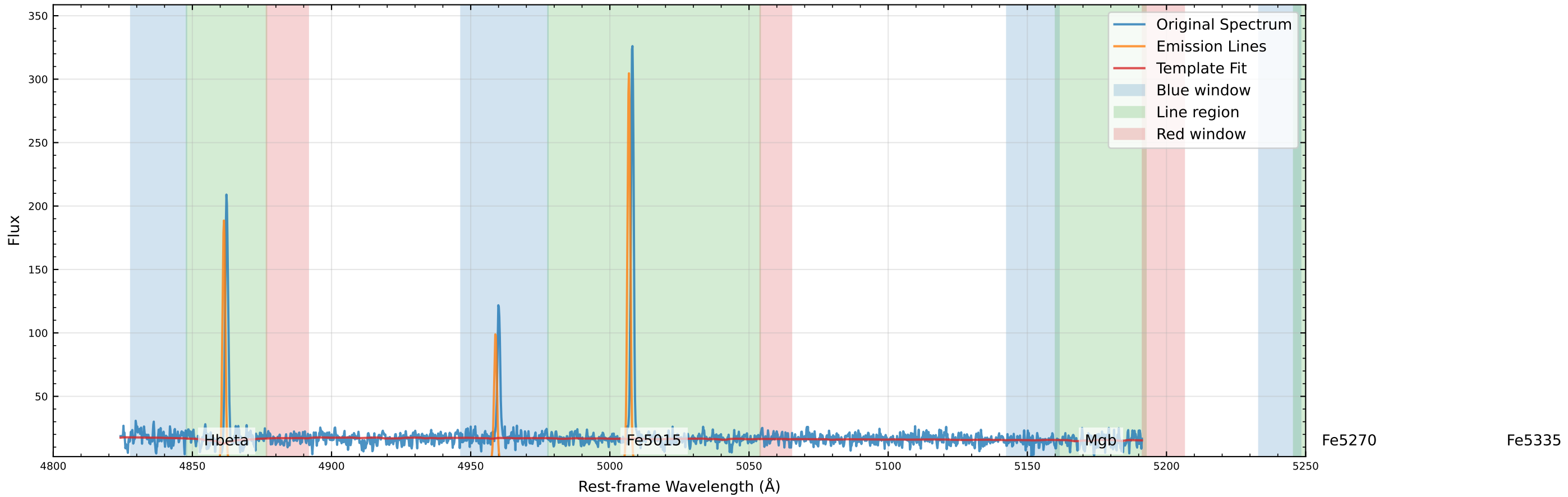
Original Data Comparison (v_star=81.2 km/s, v_gas=70.3 km/s)
