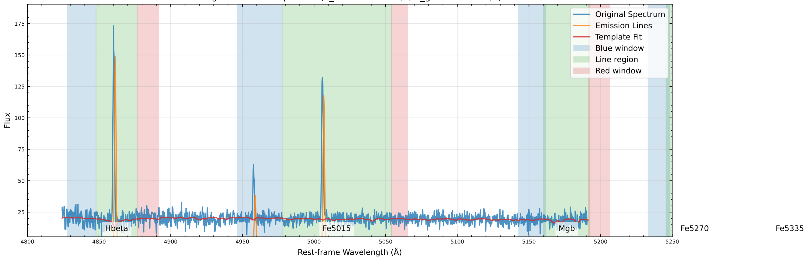
Original Data Comparison (v_star=-53.5 km/s, v_gas=-65.1 km/s)
