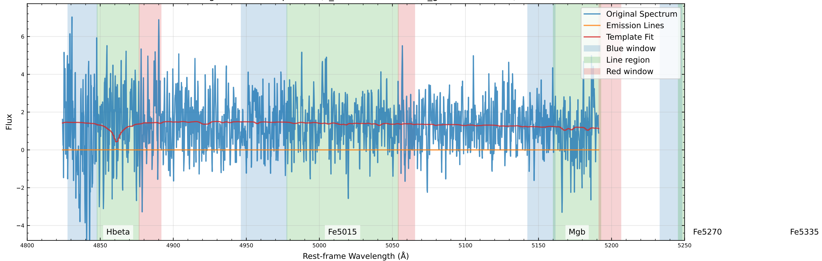
Original Data Comparison (v_star=-612.9 km/s, v_gas=-607.8 km/s)
