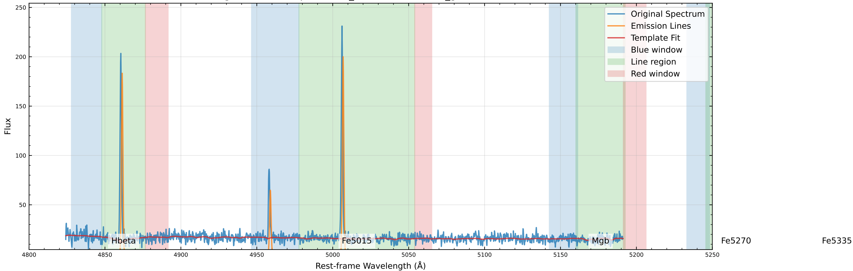
Original Data Comparison (v_star=-24.5 km/s, v_gas=-49.6 km/s)
