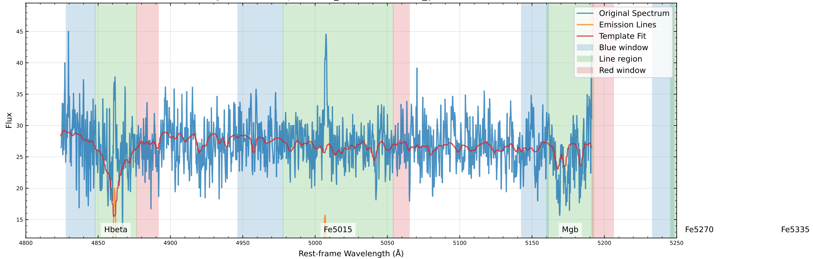
Original Data Comparison (v_star=29.6 km/s, v_gas=21.8 km/s)
