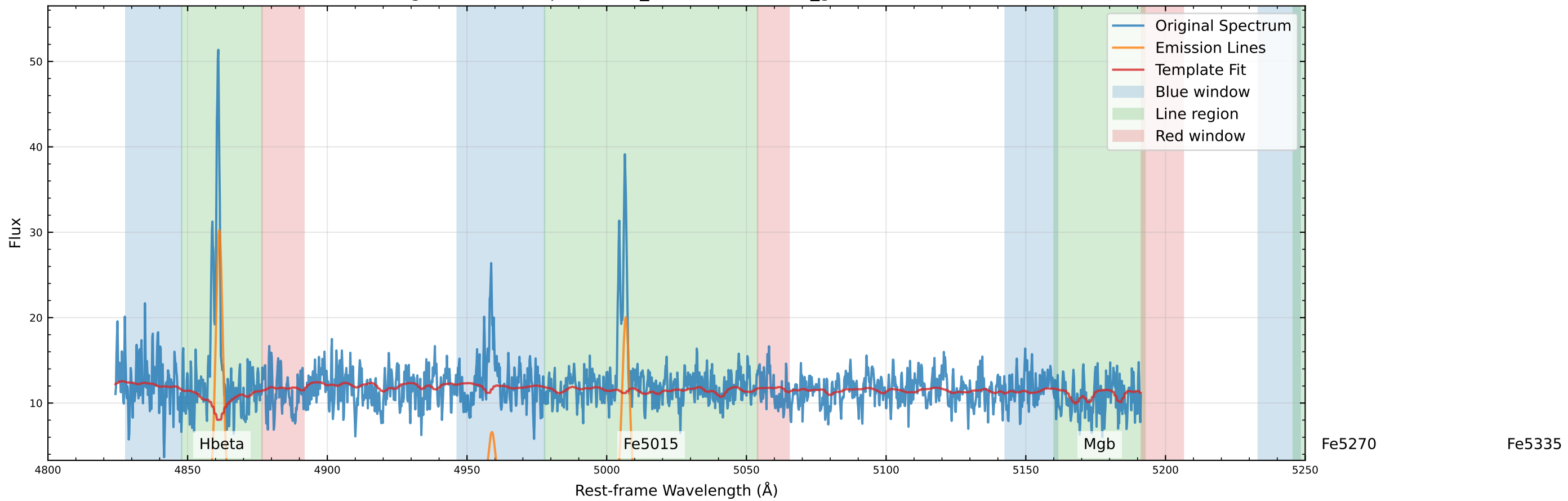
Original Data Comparison (v_star=16.4 km/s, v_gas=-44.7 km/s)
