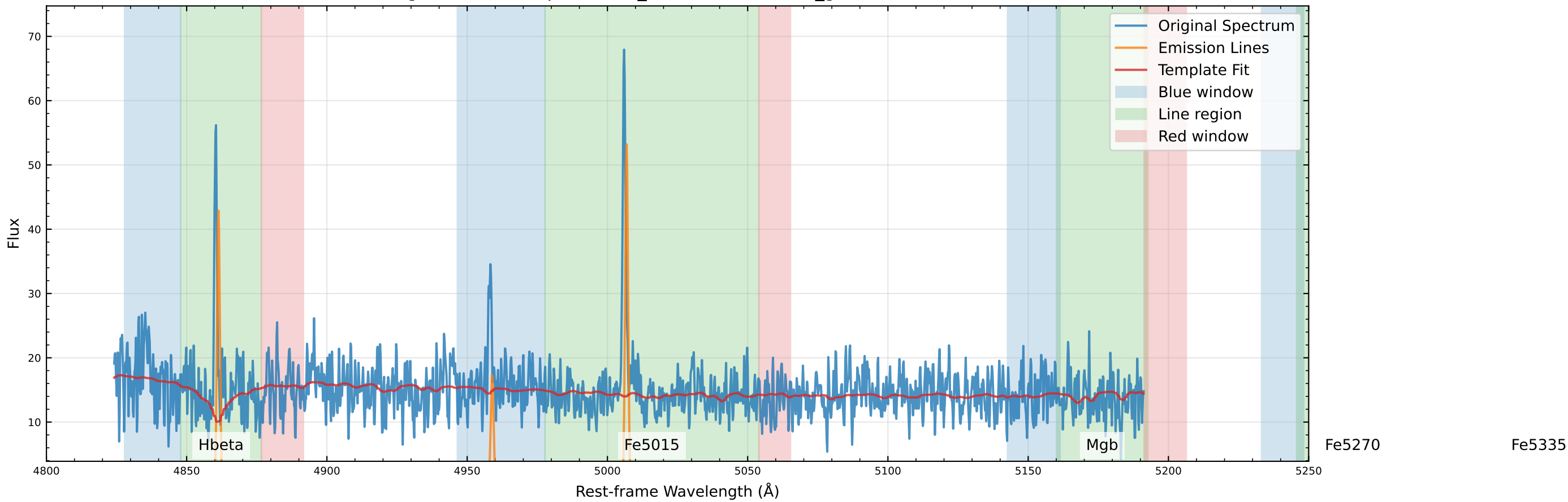
Original Data Comparison (v_star=-36.7 km/s, v_gas=-56.2 km/s)
