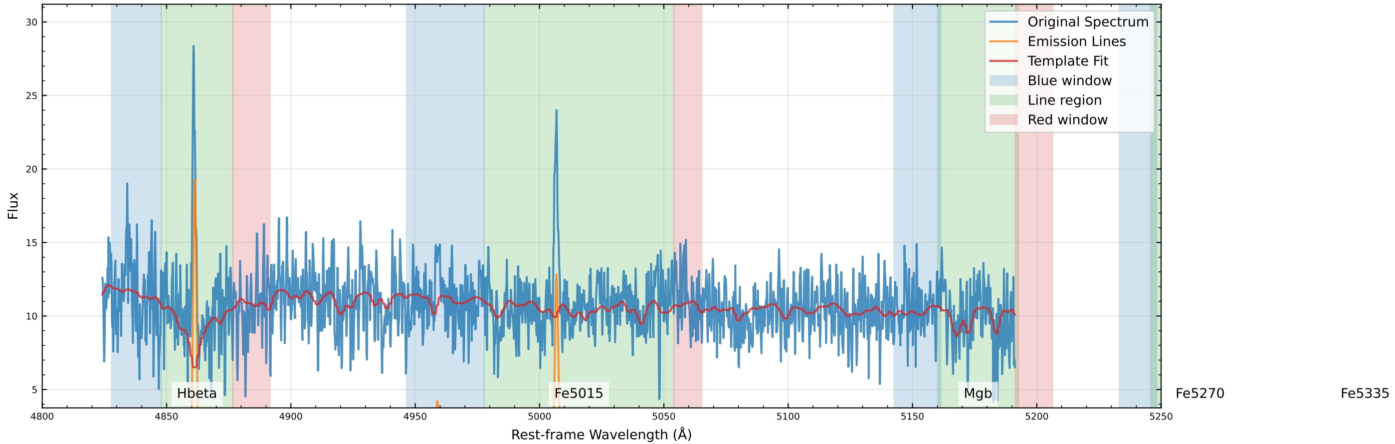
Original Data Comparison (v_star=9.4 km/s, v_gas=-16.4 km/s)
