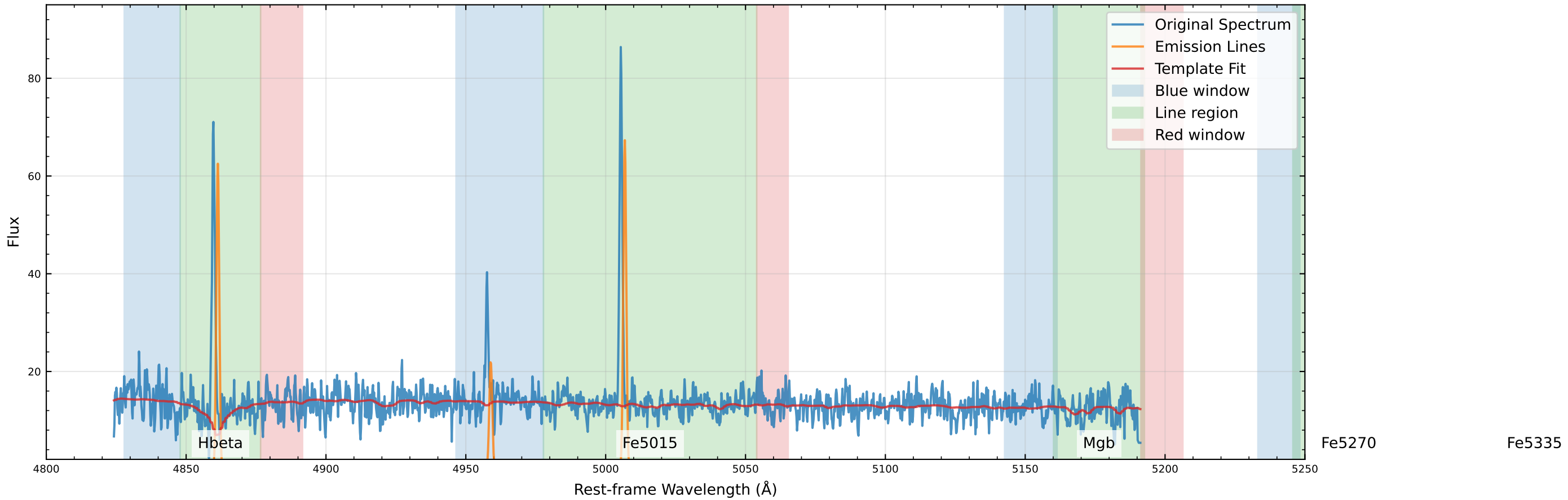
Original Data Comparison (v_star=-98.3 km/s, v_gas=-88.4 km/s)
