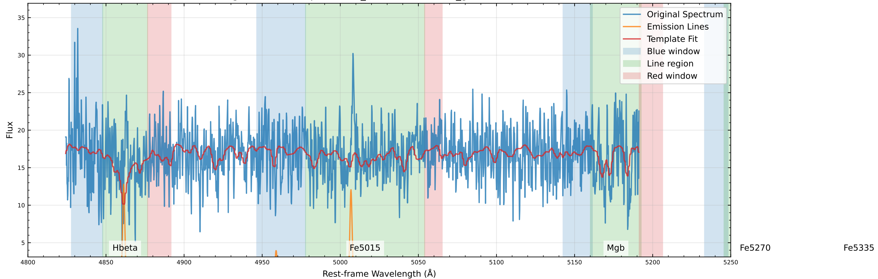
Original Data Comparison (v_star=53.3 km/s, v_gas=83.6 km/s)
