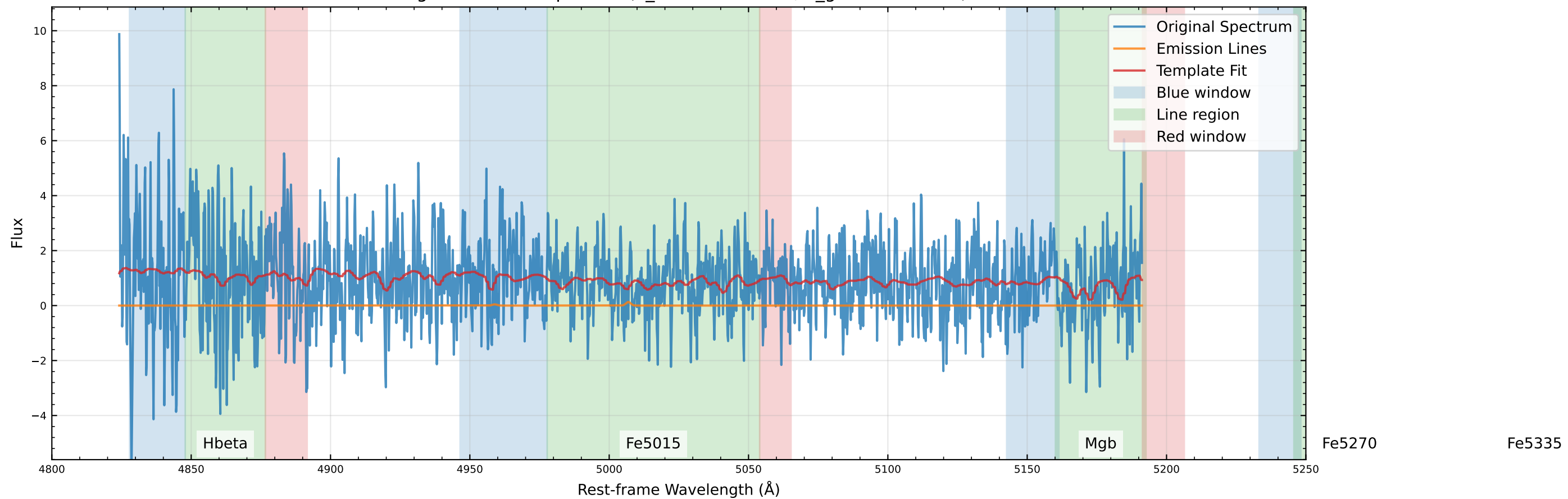
Original Data Comparison (v_star=42.9 km/s, v_gas=39.4 km/s)
