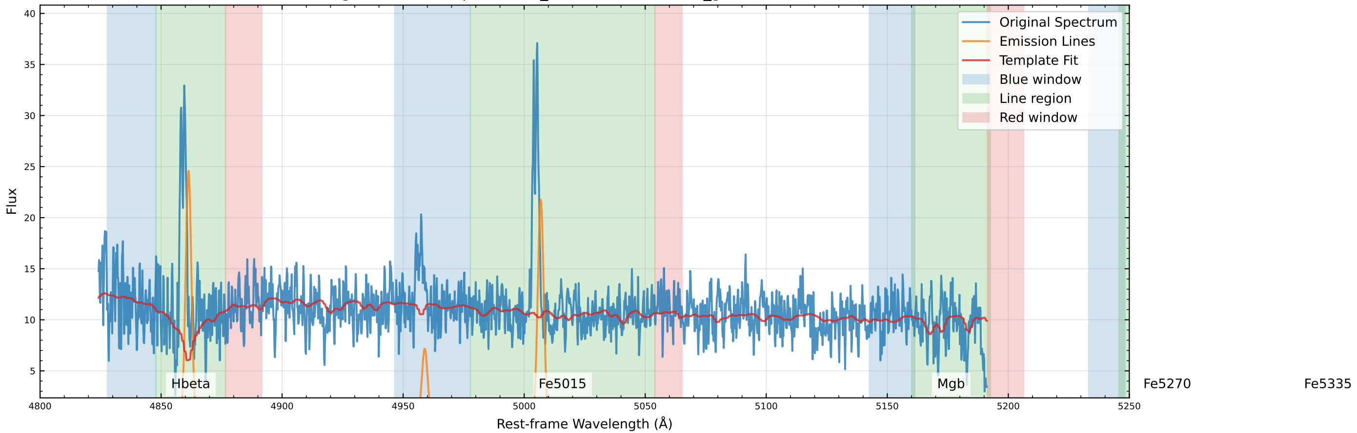
Original Data Comparison (v_star=-126.8 km/s, v_gas=-127.9 km/s)
