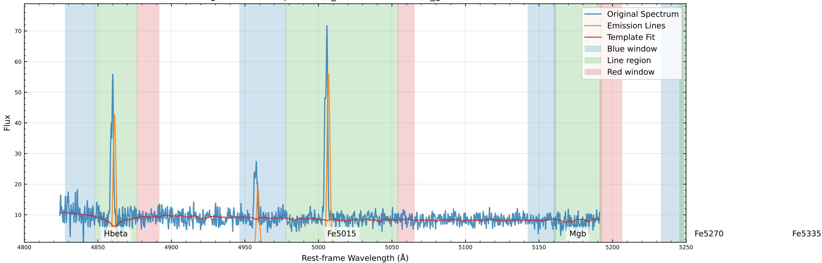
Original Data Comparison (v_star=-107.8 km/s, v_gas=-90.8 km/s)
