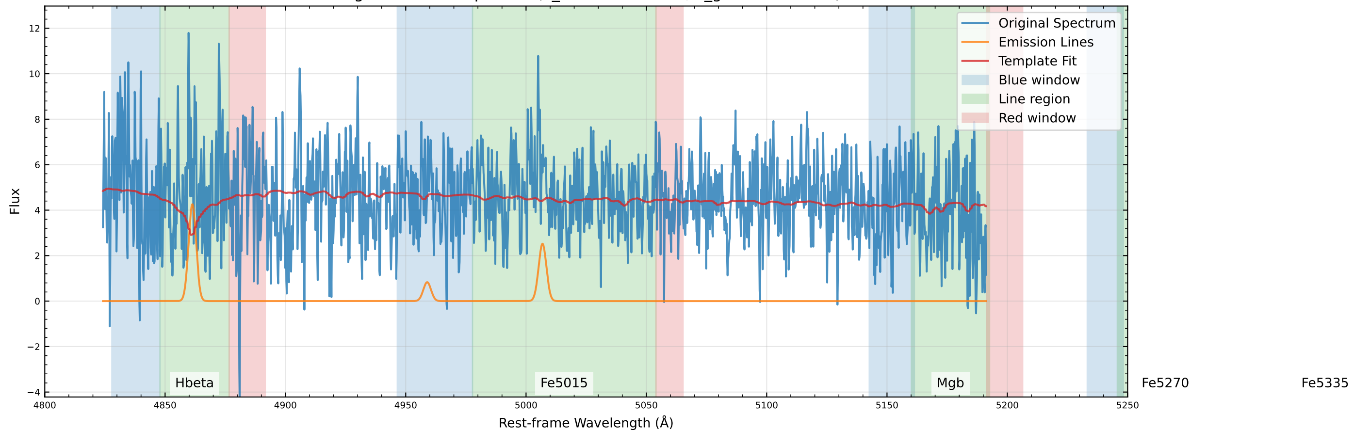
Original Data Comparison (v_star=-27.0 km/s, v_gas=-55.9 km/s)
