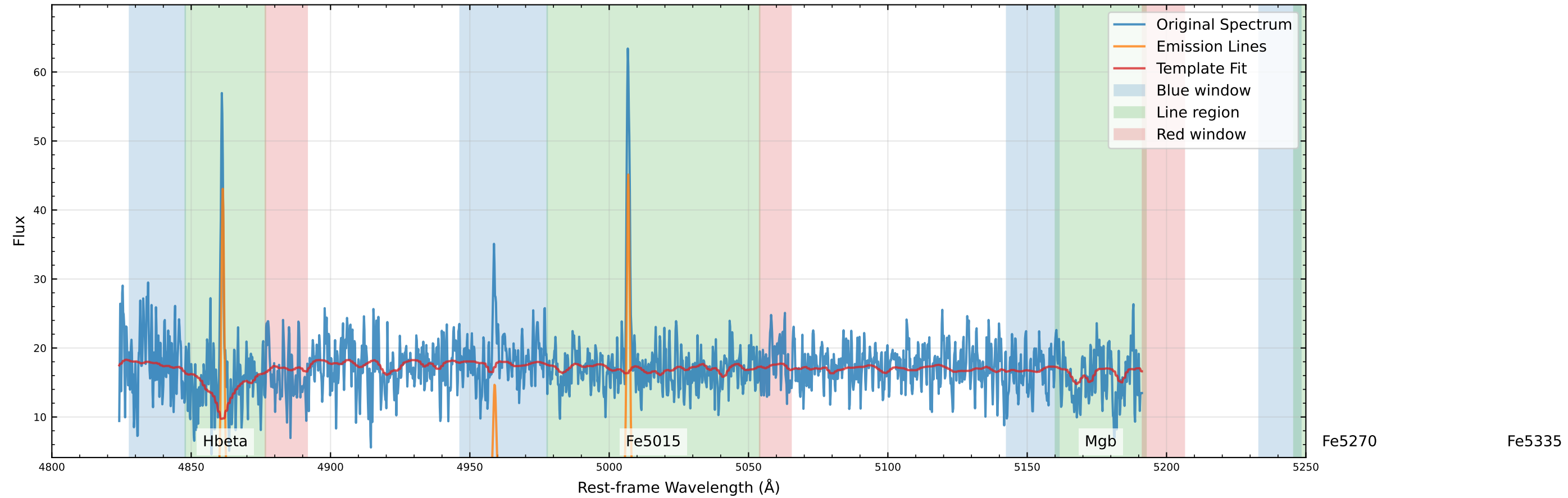
Original Data Comparison (v_star=-36.8 km/s, v_gas=-9.4 km/s)
