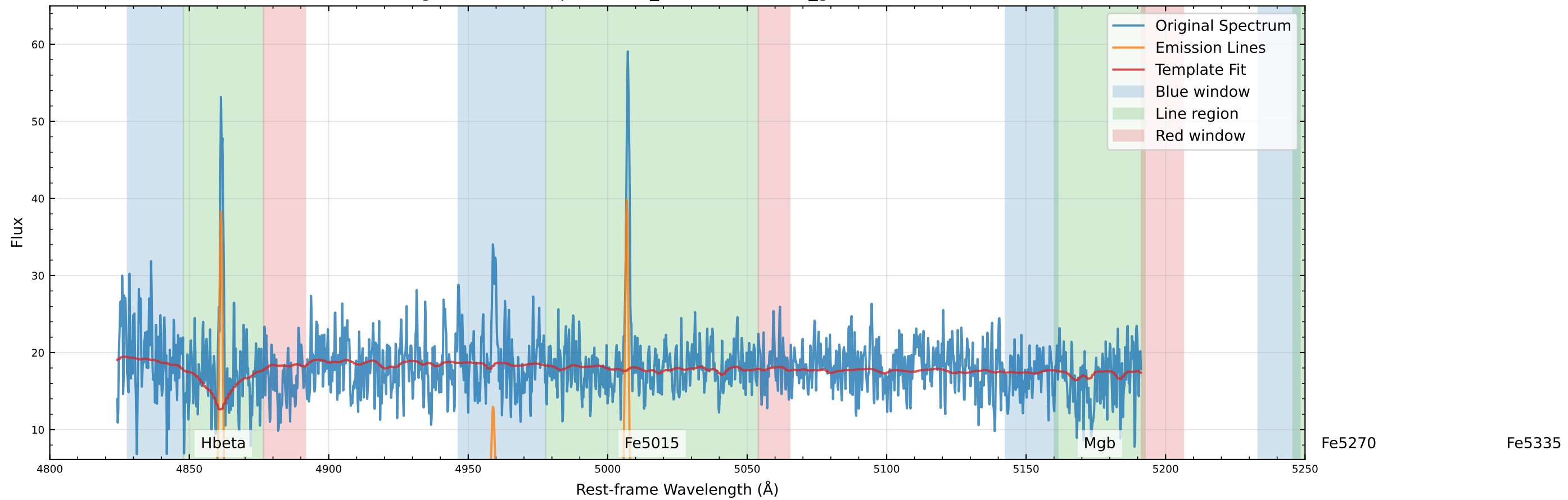
Original Data Comparison (v_star=5.8 km/s, v_gas=20.0 km/s)
