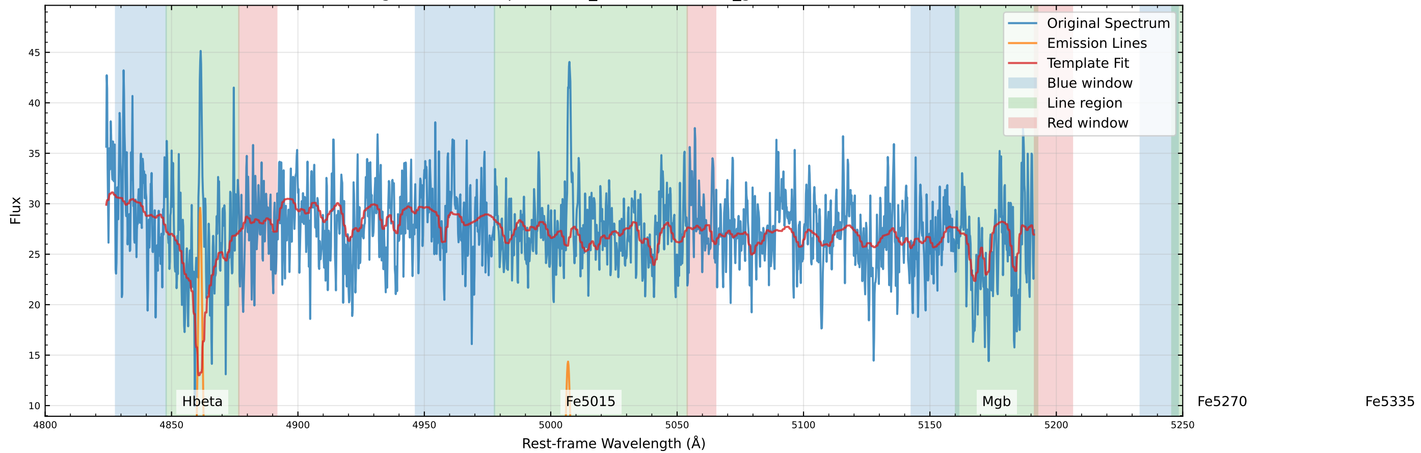
Original Data Comparison (v_star=7.4 km/s, v_gas=20.8 km/s)
