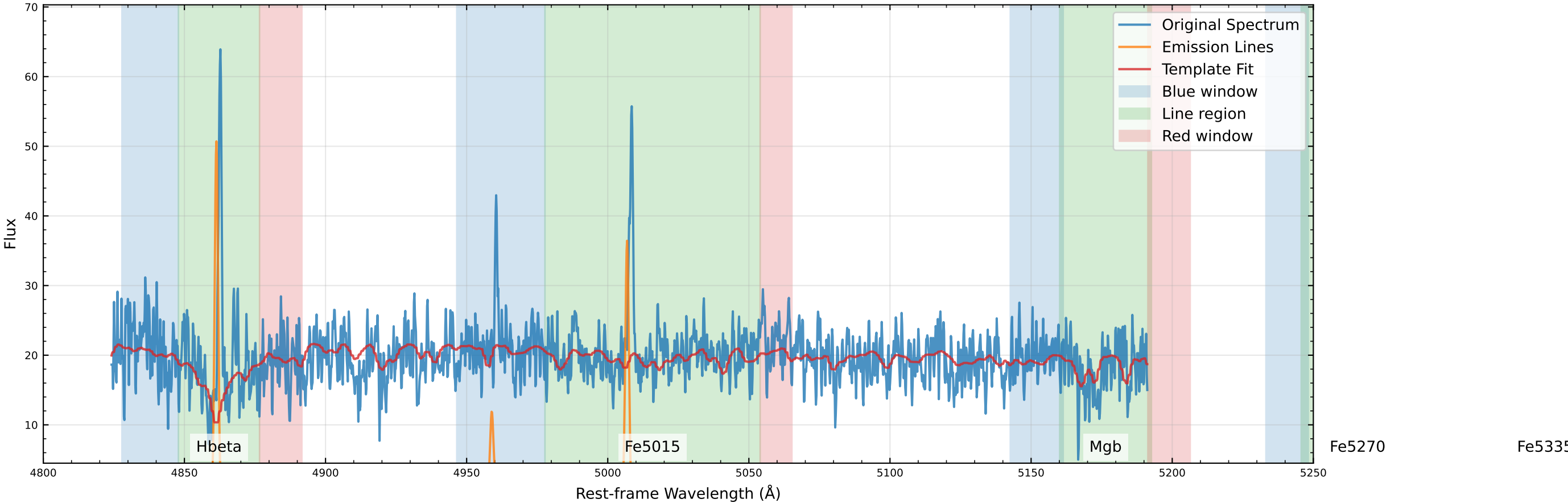
Original Data Comparison (v_star=53.3 km/s, v_gas=82.8 km/s)
