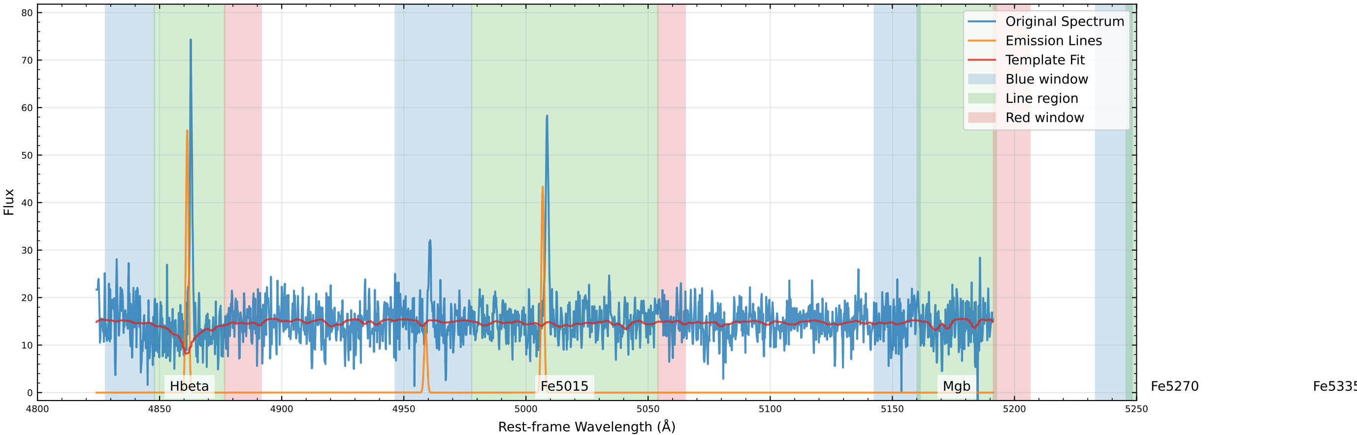
Original Data Comparison (v_star=46.7 km/s, v_gas=99.3 km/s)
