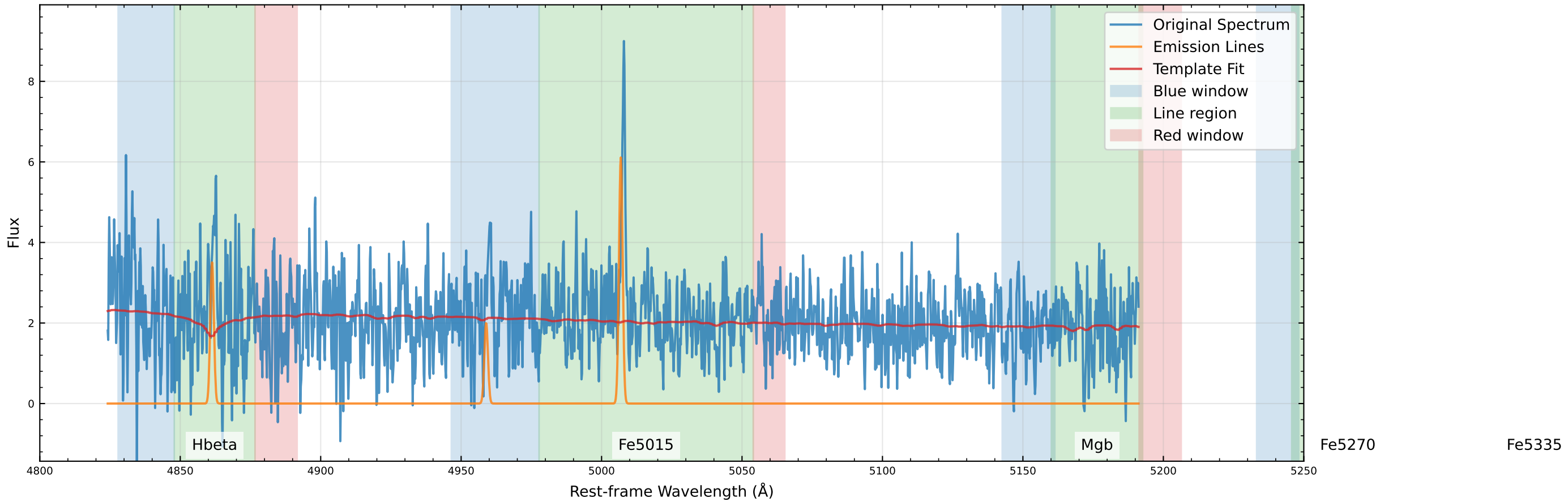
Original Data Comparison (v_star=1.4 km/s, v_gas=58.0 km/s)
