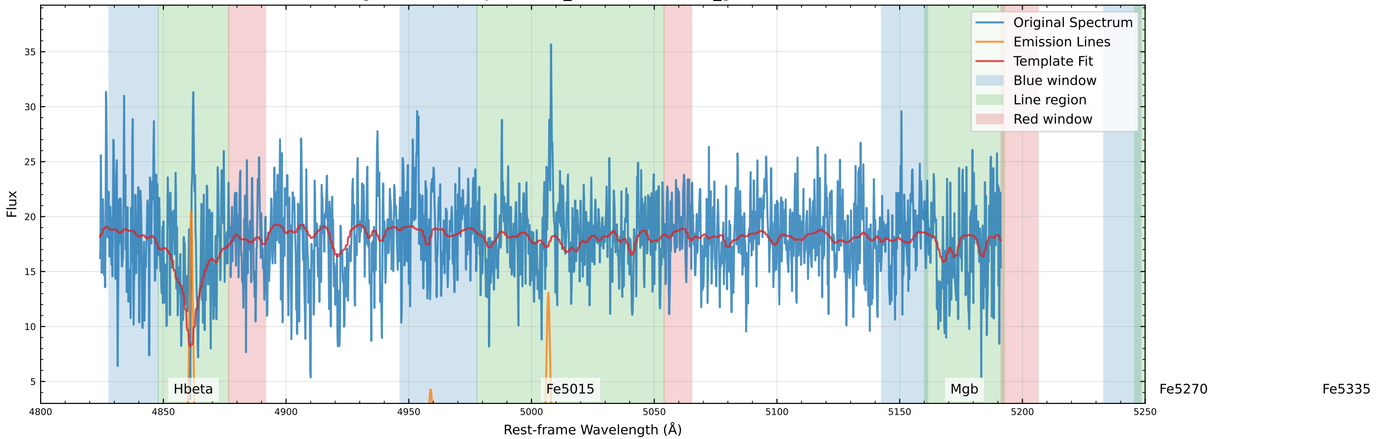
Original Data Comparison (v_star=21.4 km/s, v_gas=55.9 km/s)
