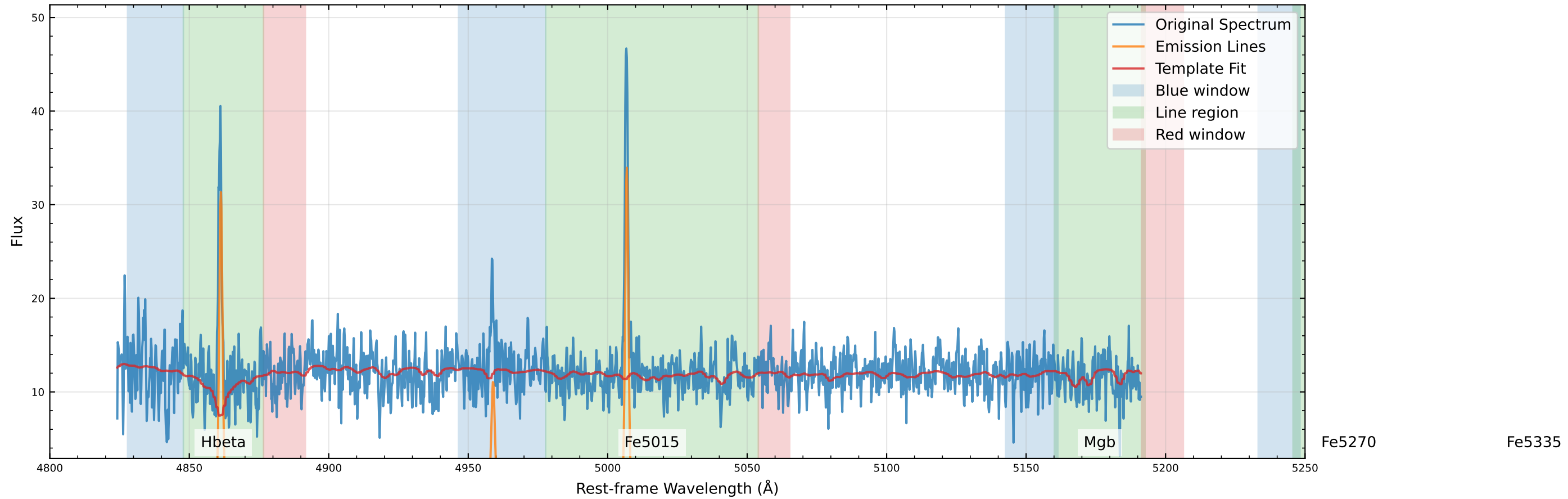
Original Data Comparison (v_star=-39.8 km/s, v_gas=-14.6 km/s)
