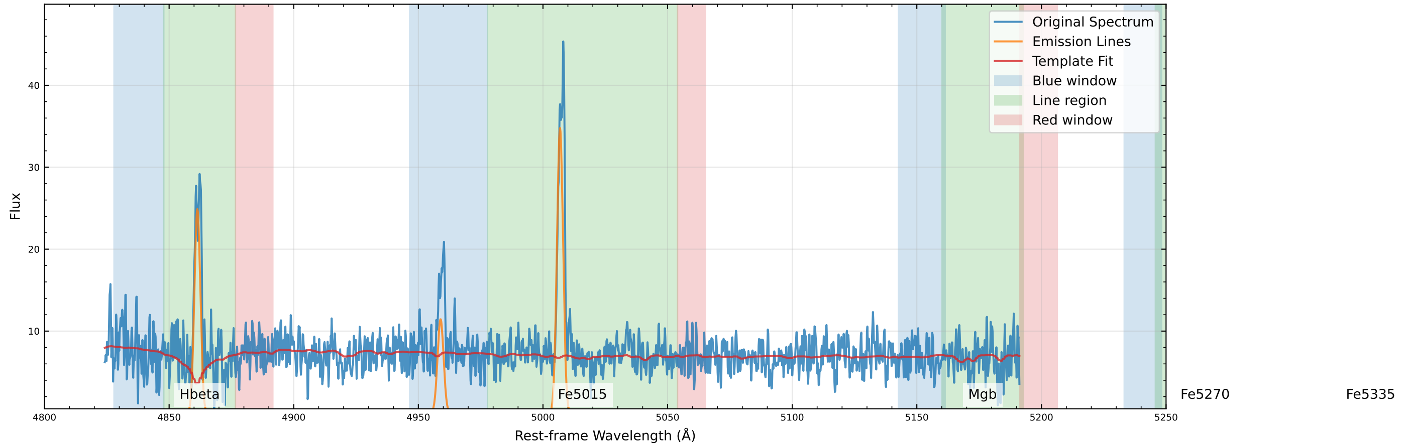
Original Data Comparison (v_star=-17.5 km/s, v_gas=34.5 km/s)
