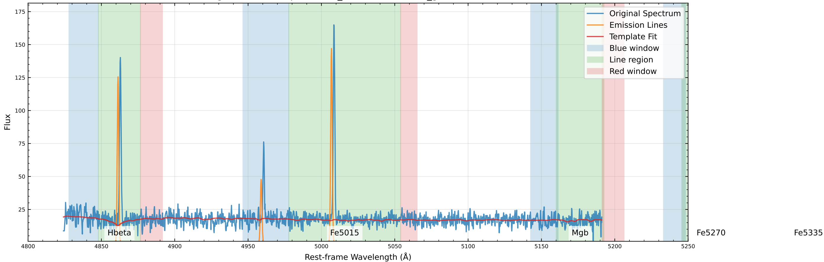
Original Data Comparison (v_star=71.2 km/s, v_gas=101.3 km/s)
