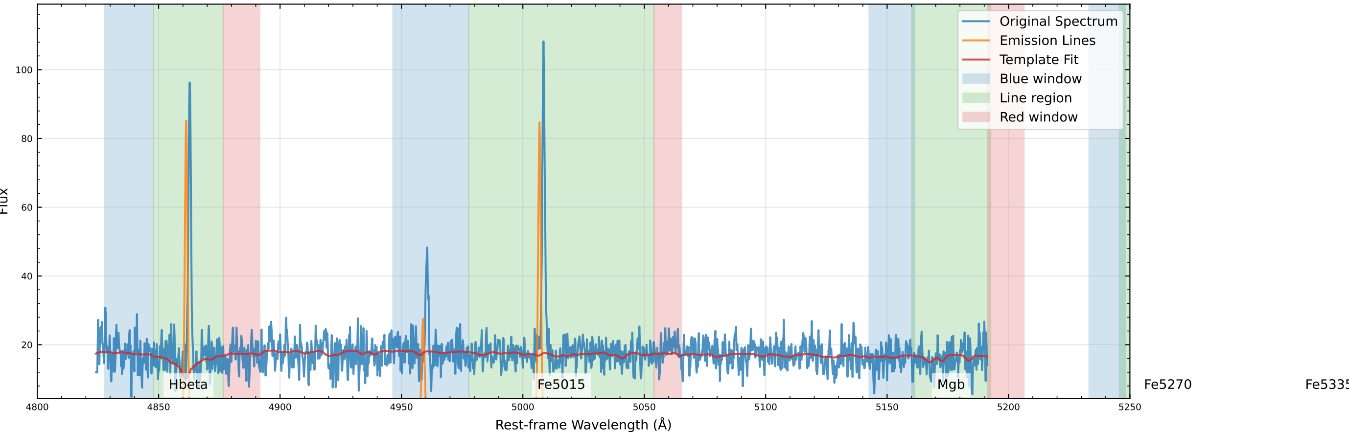
Original Data Comparison (v_star=69.2 km/s, v_gas=95.2 km/s)
