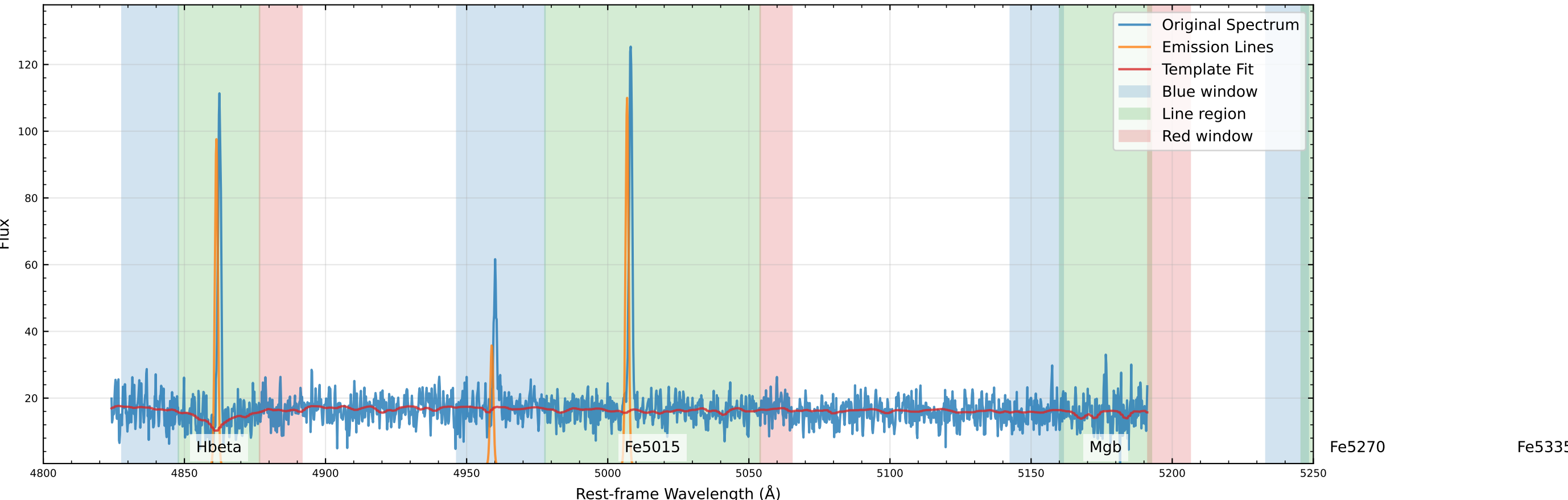
Original Data Comparison (v_star=-13.8 km/s, v_gas=72.1 km/s)
