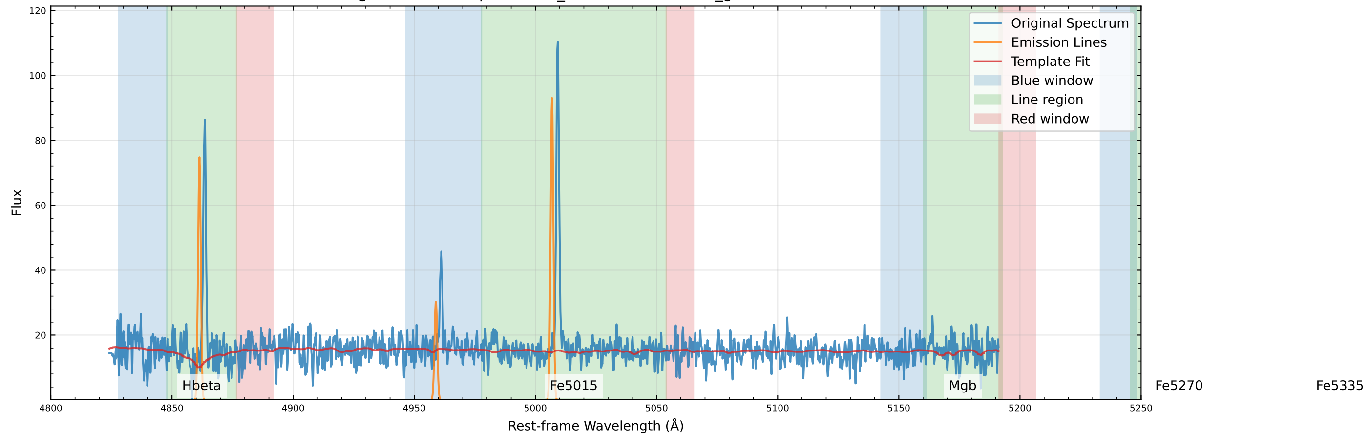
Original Data Comparison (v_star=120.2 km/s, v_gas=136.5 km/s)
